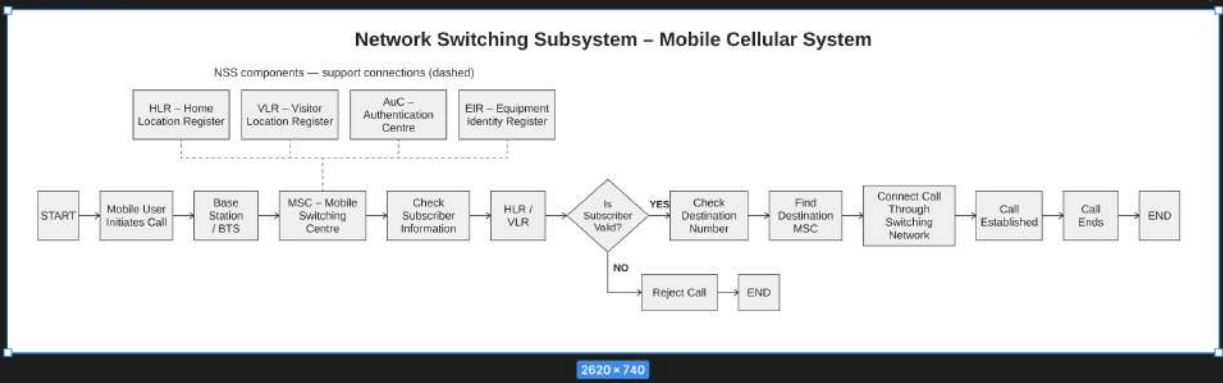
NSS horizontal call flow
